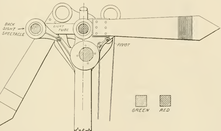
PIPER TRAIN ORDER SIGNAL WITH "BACK SIGHT."
